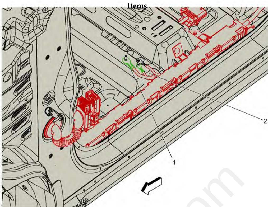
Fig. 14: G301 and G303 (LWN)
